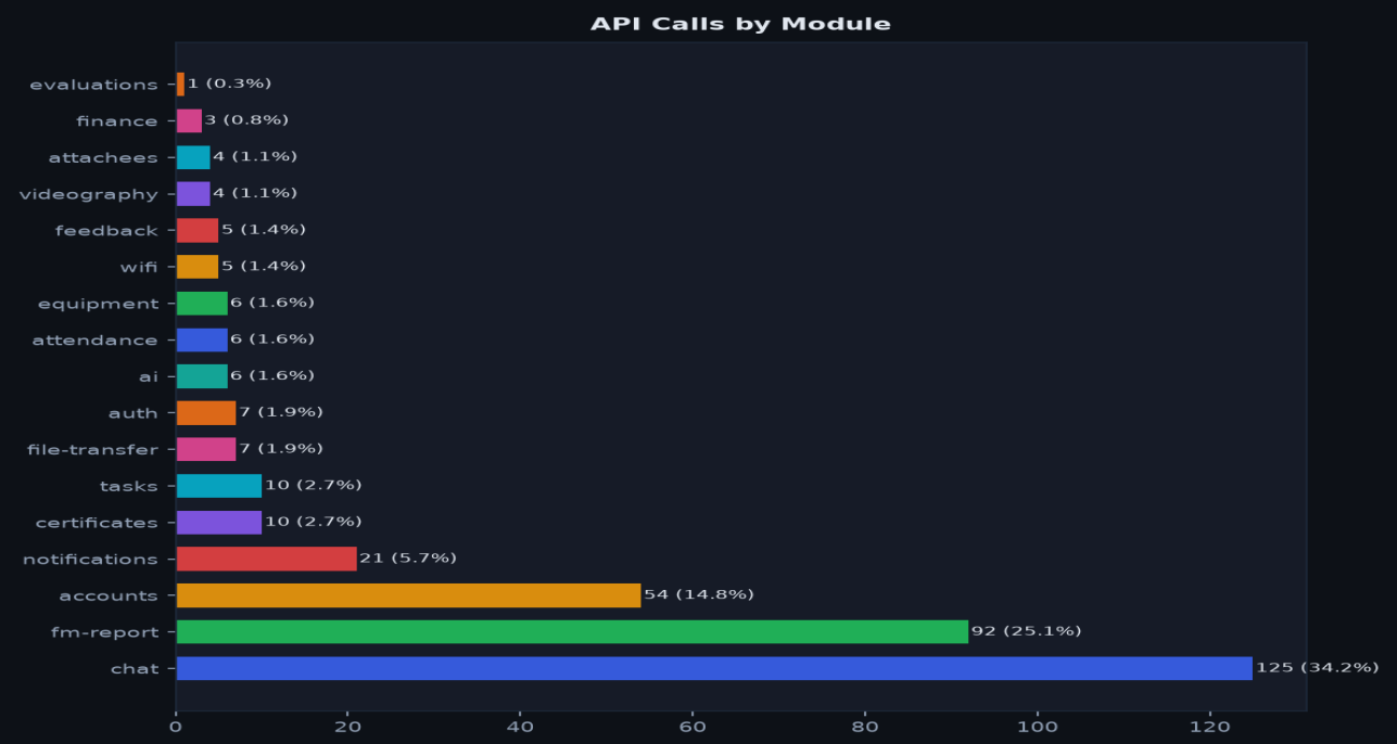
Fig 3 – API calls per module with percentage share
